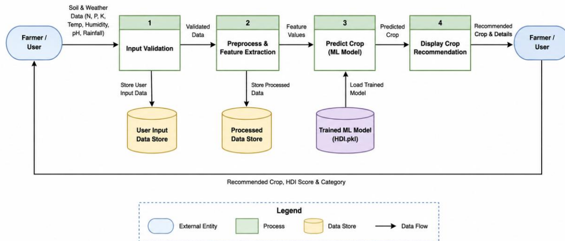
Data Flow Diagram: OptiCrop – AI Based Crop Recommendation System
